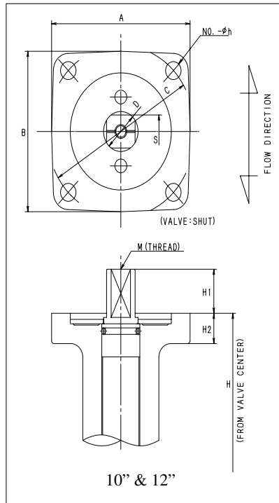
DIMENSIONS - SPECIFICATIONS
